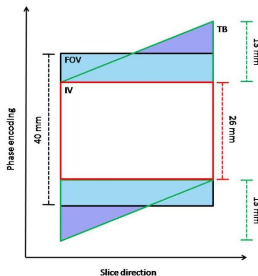
Figure 36 Schematic representation of the FOV (black rectangle, 40 mm) dimension and Tb (green rectangles, 13 mm each) influence on the final image. The desired IV (red rectangle, 26 mm) is at the center of the acquired FOV. Outside the acquired FOV, symmetrically with respect to the phase encoding direction, there are 6 mm of the Tb (violet areas). These areas cause an wraparound artifact in the remaining 7 mm of the Tb that are inside the acquired FOV (light blue
