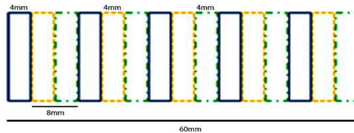
Figure 34 Schematic representation of slice order acquisition. Each color represents a group of slices. Slice thickness 4mm, gap between slices 8mm, total acquire thickness 60mm. In this example, in order not to excite contiguous slices, the whole volume is acquired by repeating three times the sequence (one time for each slice group).
